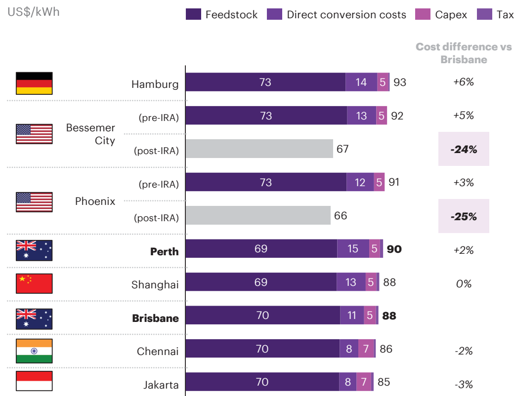
Exhibit A12: Potential production costs for packs
